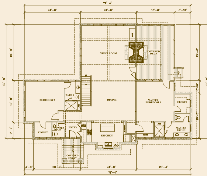
2,367 MAIN LEVEL
